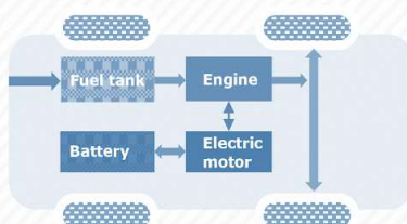
Hybrid Electric Vehicle (HEV)
