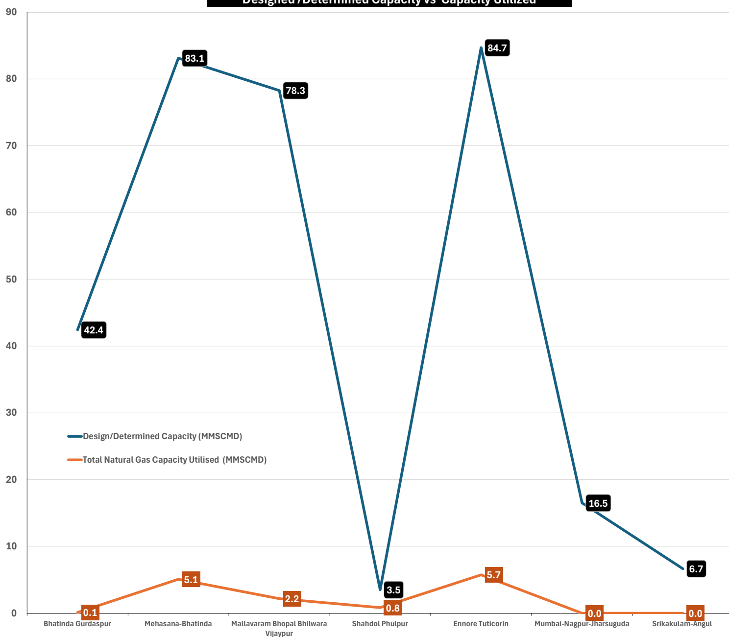
Designed /Determined Capacity vs Capacity Utilized
