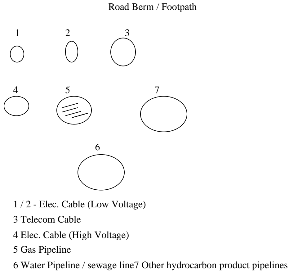
Figure 1 – Relative Position of Gas Pipeline and Distribution Mains
