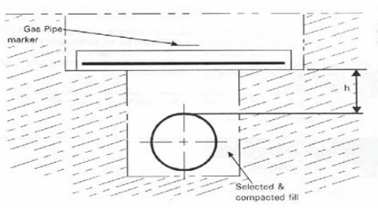
Figure 1 – Relative Position of Gas Pipeline and Distribution Mains
