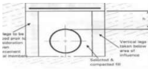
Figure 2 (b) - Concrete Slab with supports
