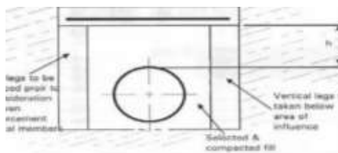
Figure 2 (b) - Concrete Slab with supports
