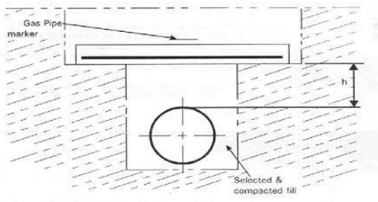
Figure 2 (a) - Concrete Slab
